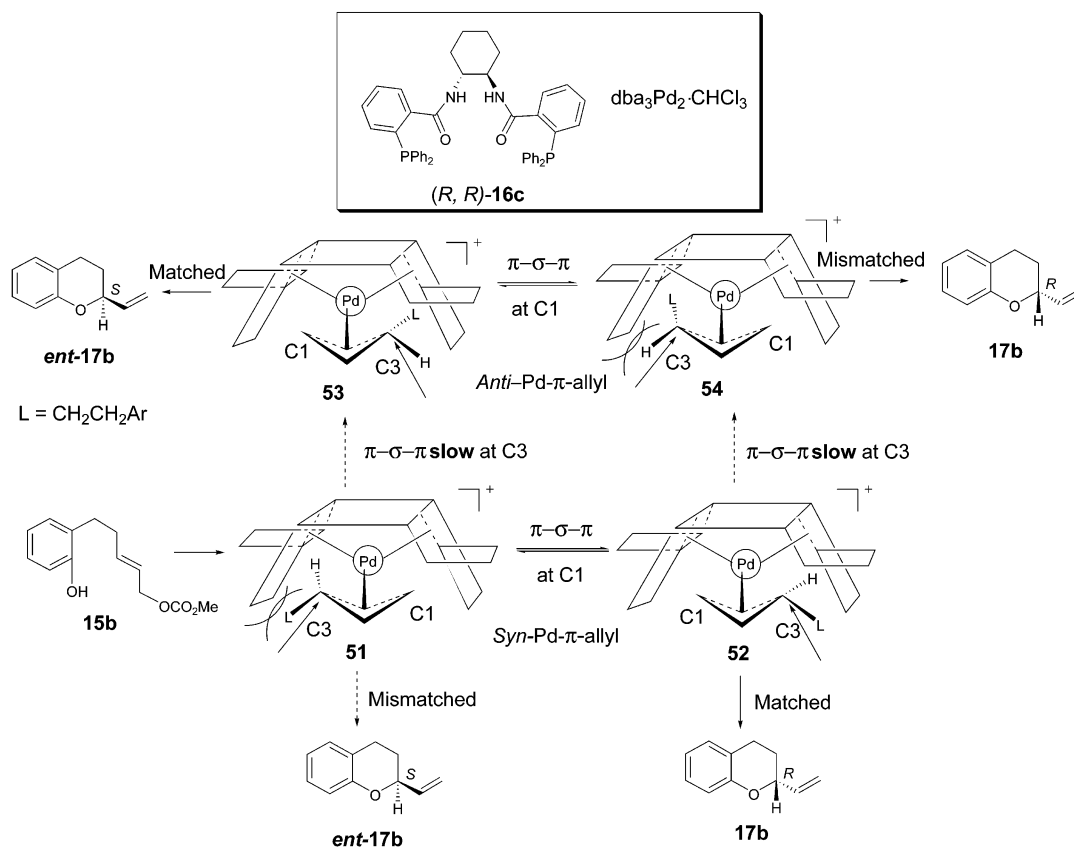
Scheme 11. Working Model for the Pd-Catalyzed AAA Reaction of Trans Disubstituted Allyl Carbonate 15b
