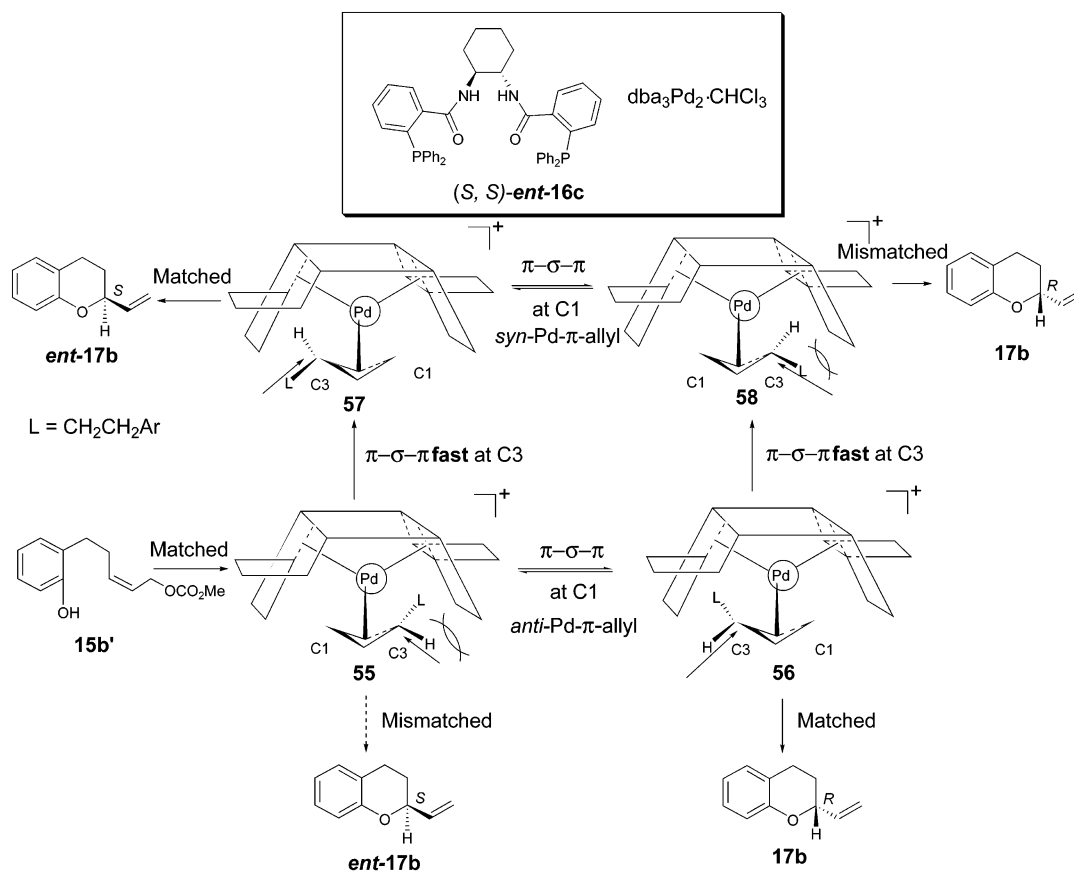
Scheme 12. Working Model for the Pd-Catalyzed AAA Reaction of Cis Disubstituted Allyl Carbonate 15b'
