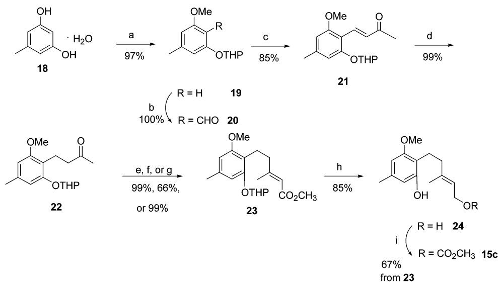
Scheme 3. First Generation Synthesis of Trans Trisubstituted Allyl Carbonate 15c a
