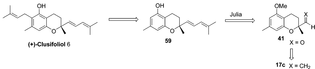
Scheme 15. Completion of Synthesis of Clusifoliol
