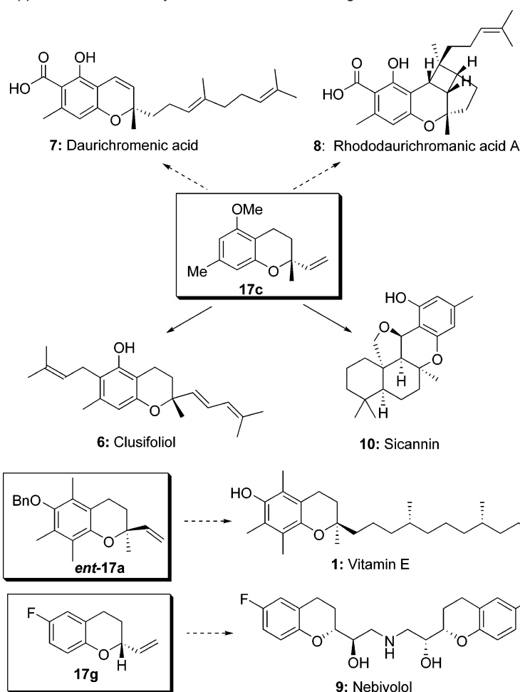
Scheme 14. Retrosynthetic Analysis of the Total Synthesis of Clusifoliol 6
