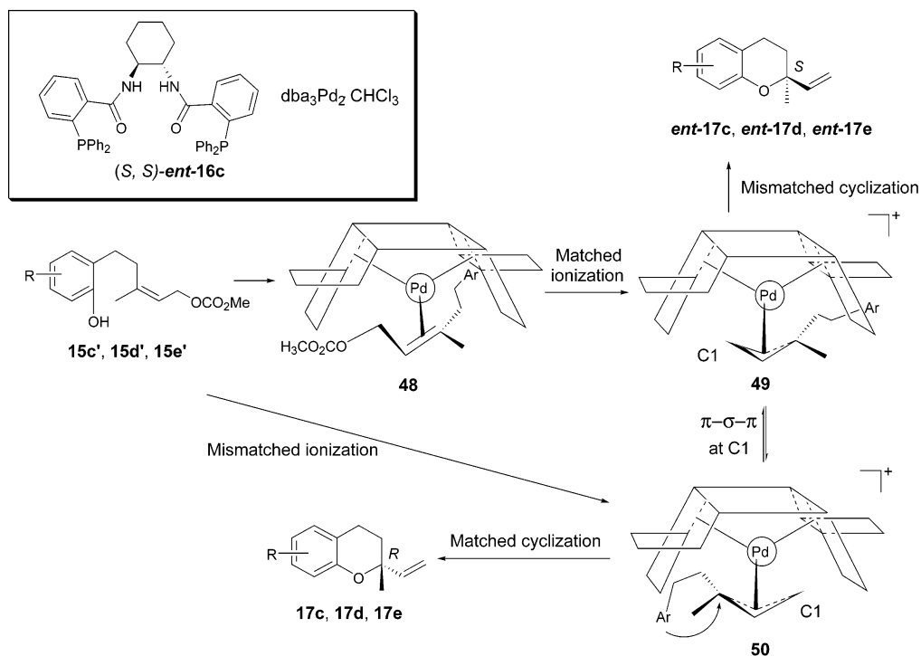
Scheme 10. Working Model for the Pd-Catalyzed Intramolecular AAA Reaction of Cis Trisubstituted Allyl Carbonates
