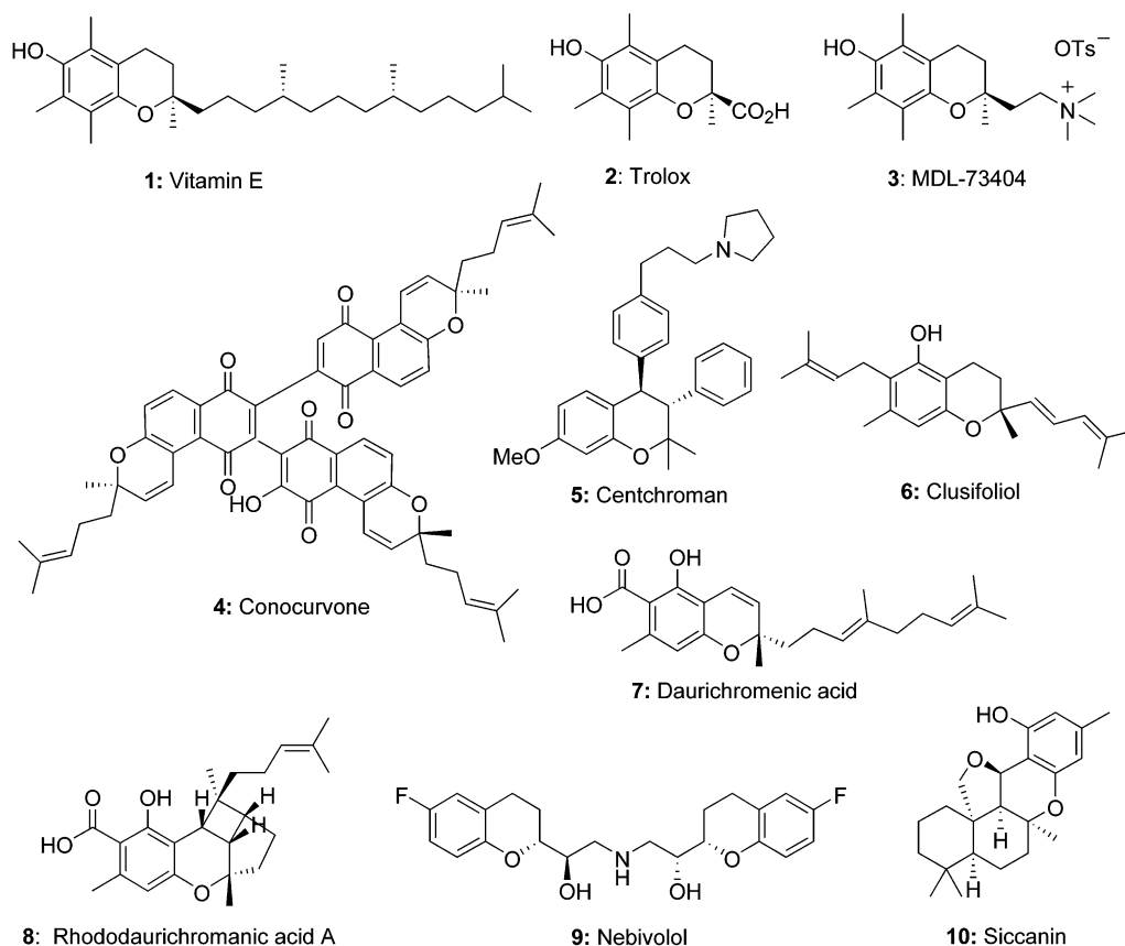
Figure 1. Representative chiral chromans and chromens.
