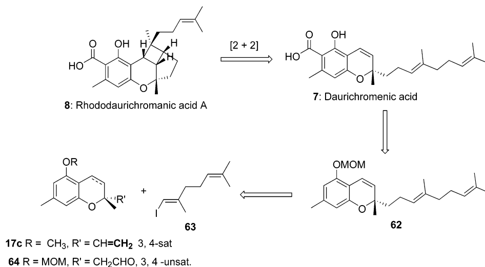
Scheme 17. Synthesis of Chromen Aldehyde 64 a
