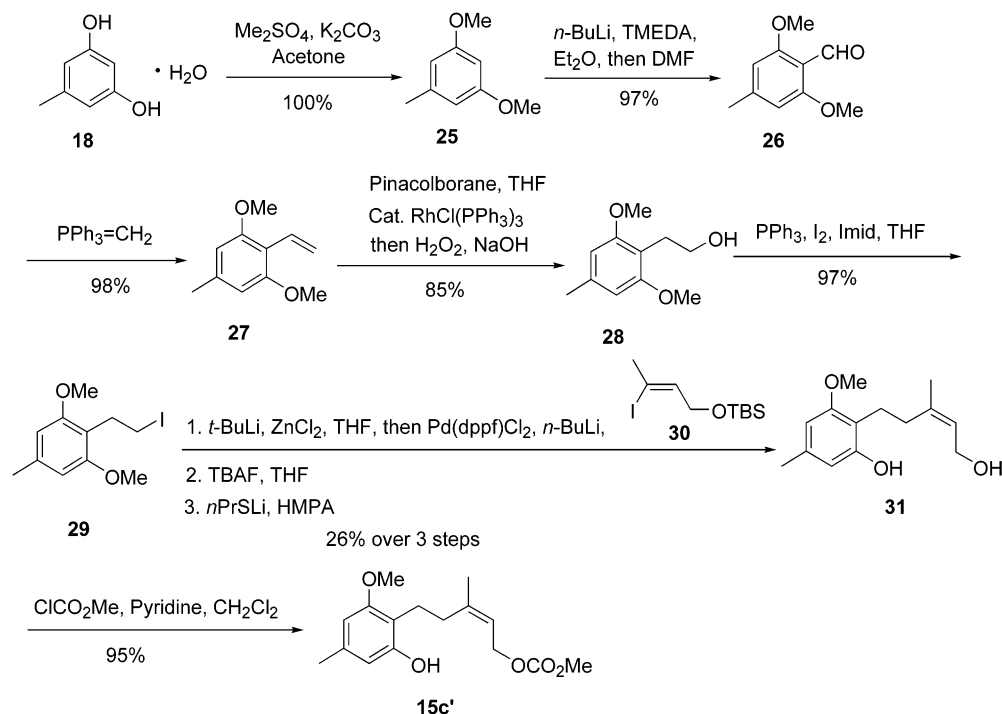
Scheme 5. Second Generation of Trans Trisubstituted Allyl Carbonate 15c
