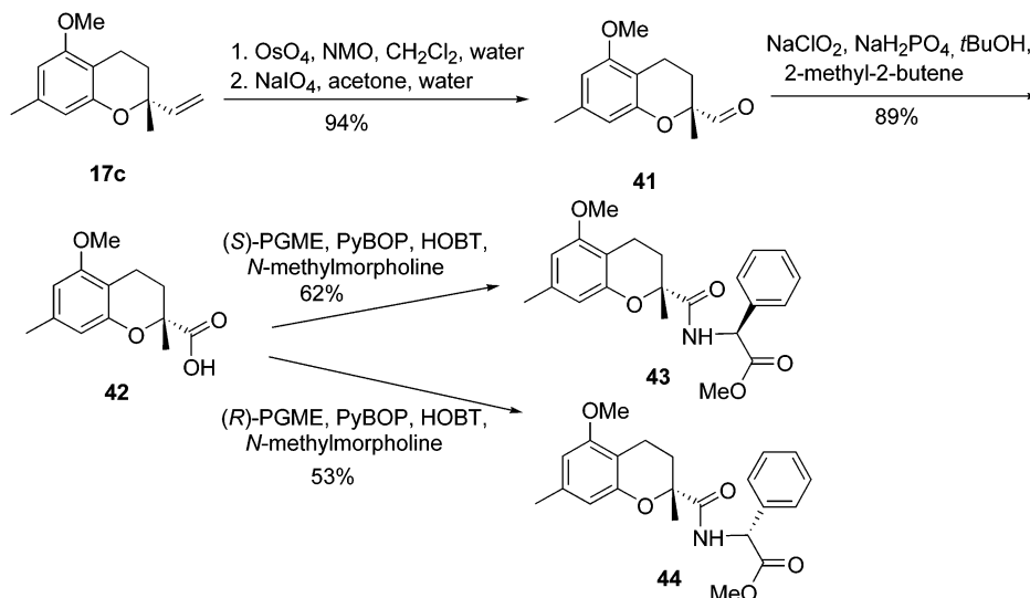
Scheme 8. Preparation of Diastereomeric Amides 43 and 44
