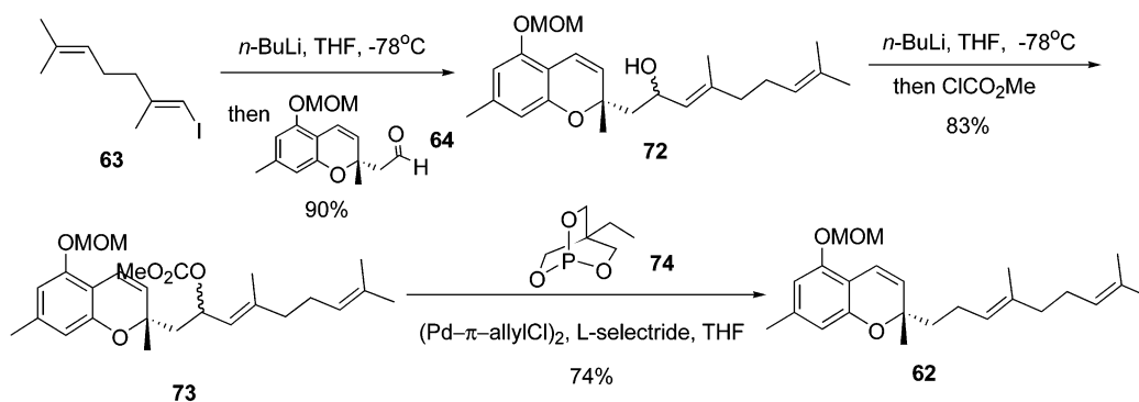
Scheme 18. Synthesis of Chromene MOM Ether 62
