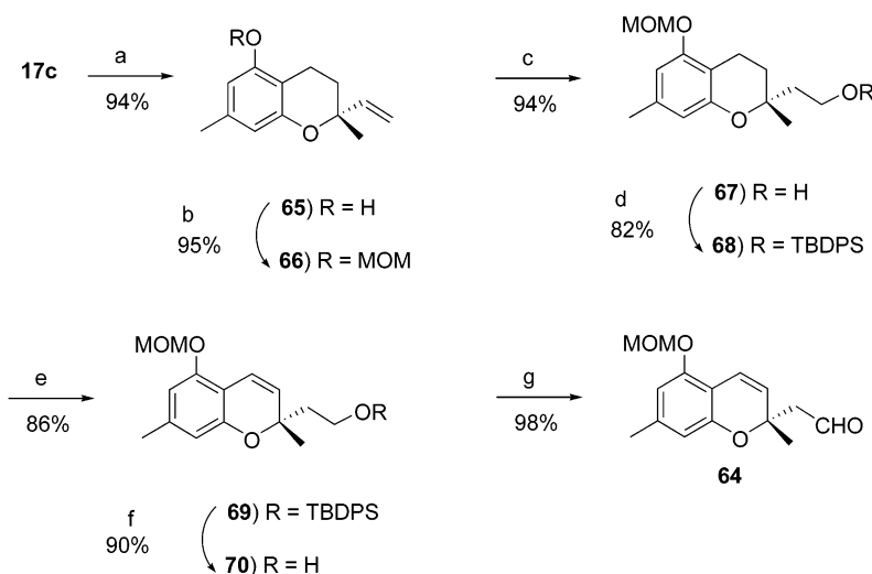
Scheme 17. Synthesis of Chromen Aldehyde 64 a
