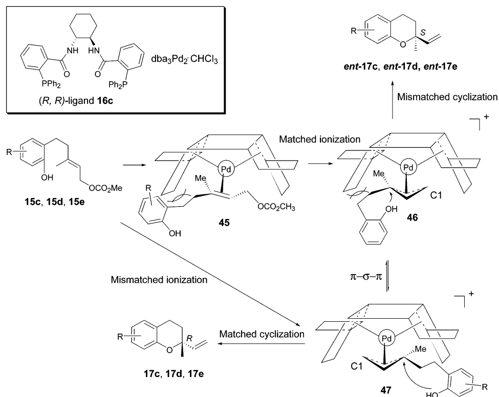
Scheme 10. Working Model for the Pd-Catalyzed Intramolecular AAA Reaction of Cis Trisubstituted Allyl Carbonates
