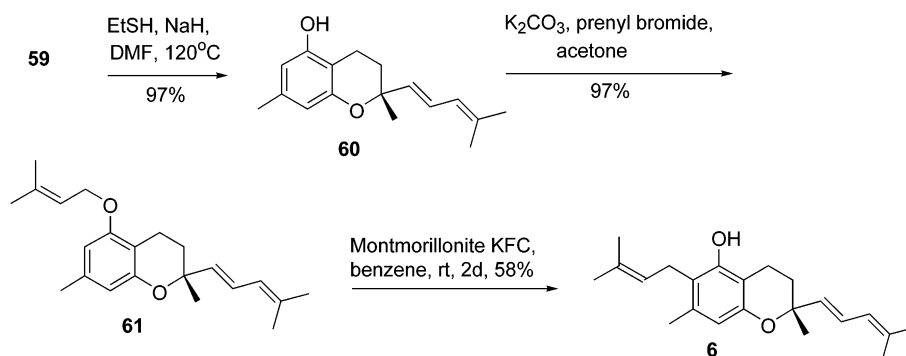
Scheme 15. Completion of Synthesis of Clusifoliol
