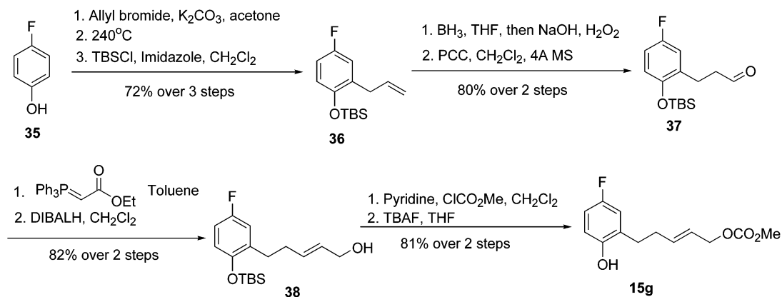
Scheme 6. Synthesis of Trans Disubstituted Allyl Carbonate 15g
