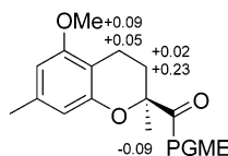
Figure 2. \Delta\delta values ( \delta_{(S)} - \delta_{(R)} ) for 10-( S )-PGME amide 43 and 10-( R )-PGME amide 44 .
